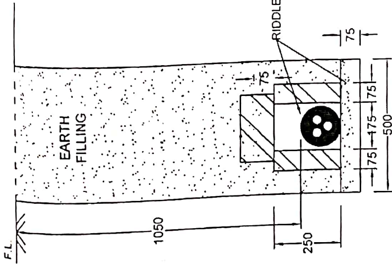
LAYING OF SINGLE CABLE IN TRENCH
